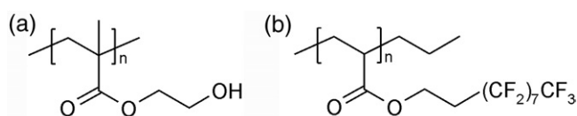
Figure 1. Structures of polymers used for surface functionalization: (a) PHEMA, (b) PFA.
