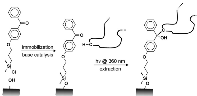
Figure 2. Schematic depiction of the surface functionalization using a photoactive benzophenone group bearing monochlorosilane.
