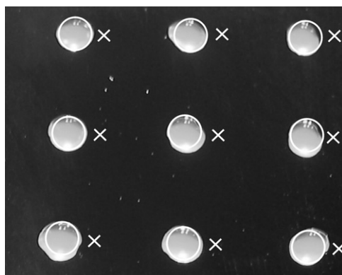
Figure 13. Photograph of an array where nine droplets impacted on nine hydrophilic spots (white rings) with a diameter of 3 mm. The impact positions had an x -offset of 2 mm (white crosses).
