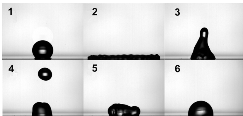
Figure 5. Impact experiment on a homogeneously coated PFA surface.
