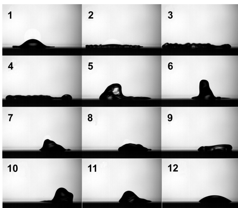
Figure 8. Impact experiment on a PFA coated substrate with a hydrophilic spot of 6 mm diameter. The centre of the hydrophilic spot is shifted 5 mm with respect to the impact centre.
