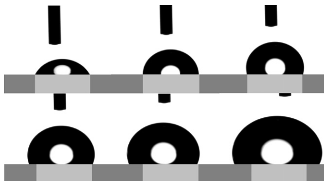
Figure 6. Video images of water drops on a PFA coated substrate with a hydrophilic spot (light grey) of 3 mm diameter. The drop volumes used are 1, 2, 3, 4, 5 and 8 \mu\text{l} .
