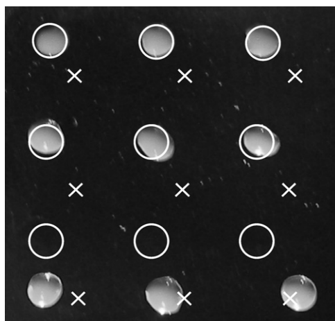
Figure 14. Photograph of an array where nine droplets impacted on the positions marked with a cross. Six out of nine droplets self-centred on hydrophilic spots. Three drops sit on the hydrophobic PFA coating.
