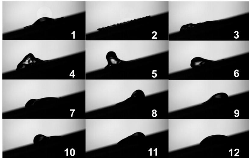
Figure 10. Impact experiment on a PFA coated surface with a hydrophilic spot of 6 mm diameter. The drop impacts 1.5 mm below the centre of the hydrophilic region. The substrate has an inclination of 15°.
