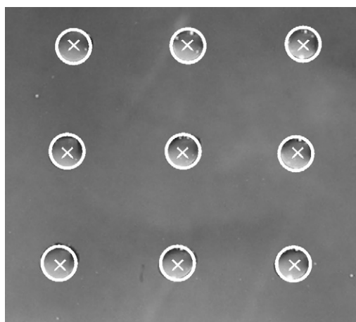
Figure 12. Photograph of an array where nine droplets impacted on nine hydrophilic spots with a diameter of 3 mm. The central impact positions are marked with a white cross.
