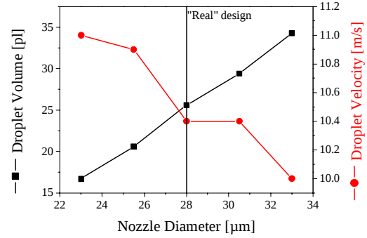
Figure 10: Simulated effect of varying the nozzle diameter on the droplet volume and velocity.
