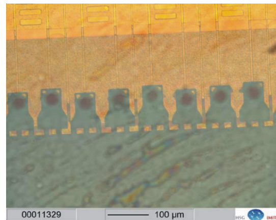
Figure 5: Assembled nozzle plate on printhead substrate. The dark areas are ink filled cavities, whereas the light areas represent leak-proof joined areas.
