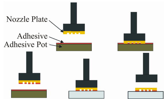
Figure 4: Schematic illustration of the adhesive transfer process.
